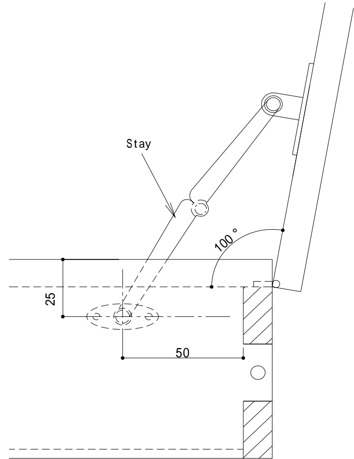
Stay Mounting Position
