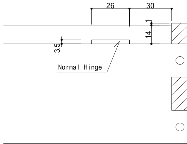
Normal Hinge Mounting Position
